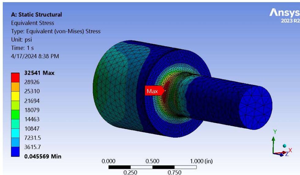
Figure 10. The stress plot for the pin with no inner hole.
