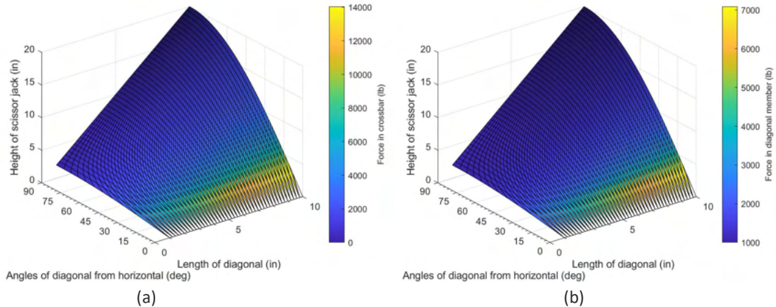
Figure 3. Surface plots show the force in the (a) crossbar and (b) diagonal member as a function of height and operating angle.
